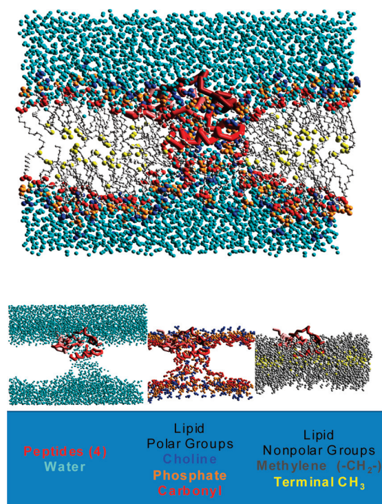
Figure 6. Molecular dynamics simulation of peptide pore formation from Sengupta and Marrink (65). (Top) The peptide-lipid bilayer with CH 2 groups removed. Blue spheres are water molecules, and yellow spheres are the terminal methyl groups. Other color spheres are the lipid polar groups. (Bottom) The same peptide-lipid bilayer separated into groups. Notice that in the vicinity of the peptide “pore” the strict segregation between polar and nonpolar is broken down.
