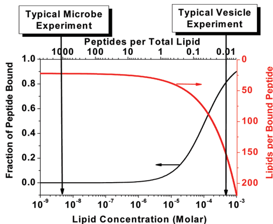
Figure 5. Typical peptide to lipid ratios in vesicle leakage experiments and microbe sterilization assays. Microbe sterilization assays are performed under conditions of peptide excess over lipid such that the membrane is saturated by peptide and there is a large reservoir of unbound peptide. Vesicle leakage experiments are done under conditions where lipid is in excess and most peptide is bound.
