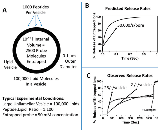
Figure 4. Release of vesicle-entrapped probes. A) A large unilamellar vesicle of 0.1 \mu\text{m} LUV, the type used in most experiments, is made of roughly 10^5 lipids enclosing a volume of about 10^{-19} liter. B) Predicted kinetics of probe release from large unilamellar vesicles containing a single pore of 10 \text{\AA} diameter. Complete release occurs in a few tenths of a second. C) Actual release kinetics observed in experiments with AMPs. Note the difference in x-axis scale indicating that actual release data is 3 orders of magnitude slower than predicted. Furthermore, the simulated release goes to completion, whereas the actual release is incomplete.
